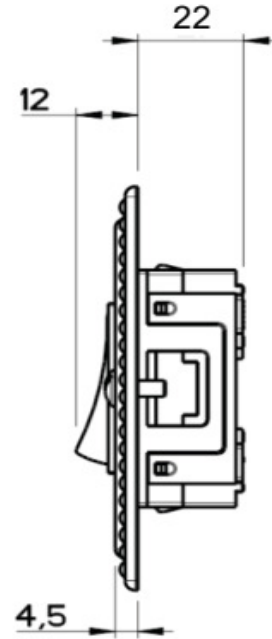
Side view common to all sizes
