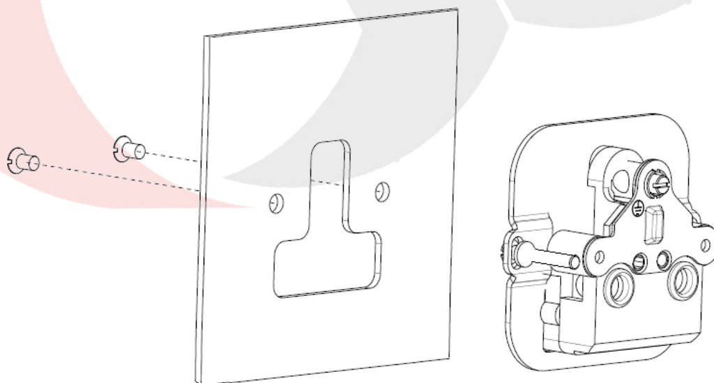
Exploded view of The Classic Square Corner Collection fixing method.
