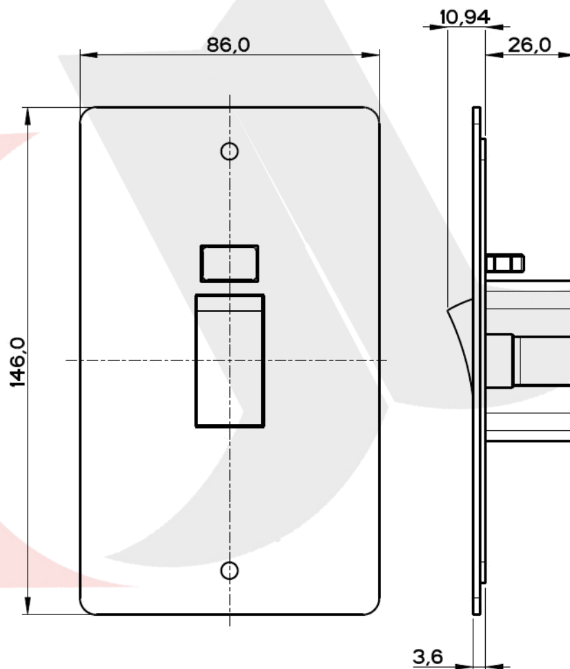
Twin 45amp Double Pole Switch
