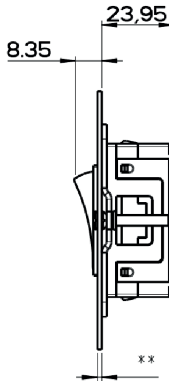
Side view common to all sizes
