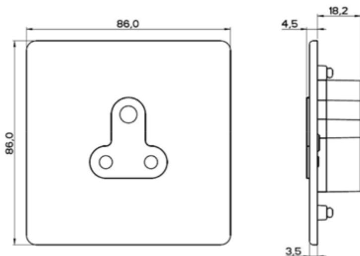
Side view common to all sizes
