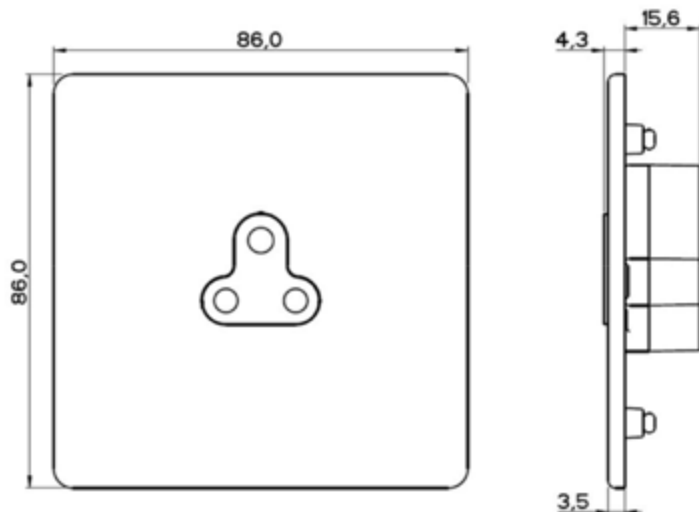
Side view common to all sizes
