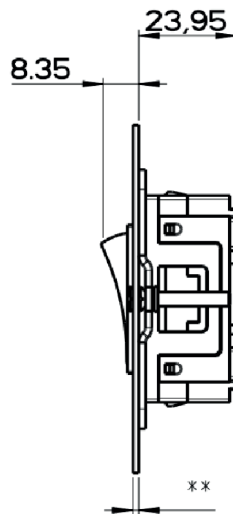
Side view common to all sizes
