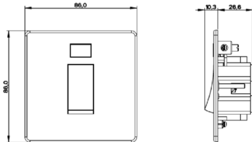
Side view common to all sizes
